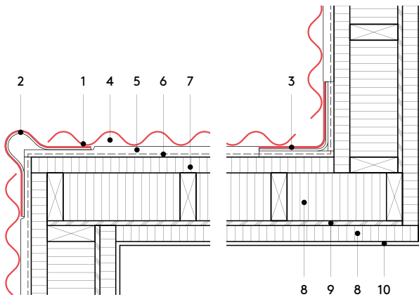
Horizontal section 1:20
