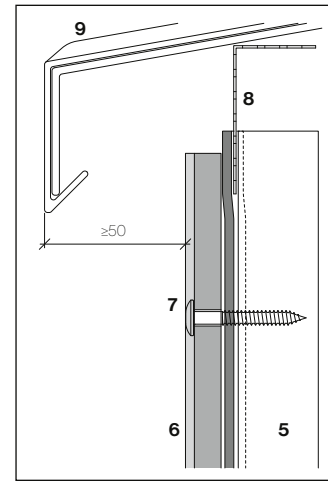
Sill detail
