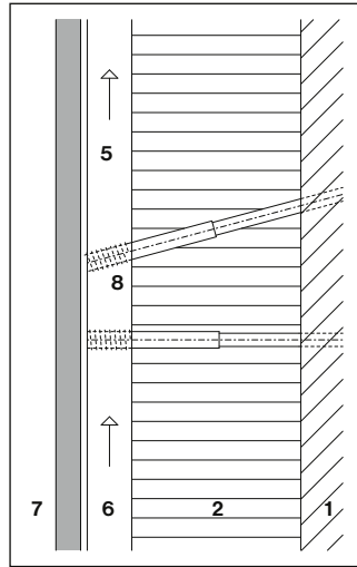
Timber / spacer screw
