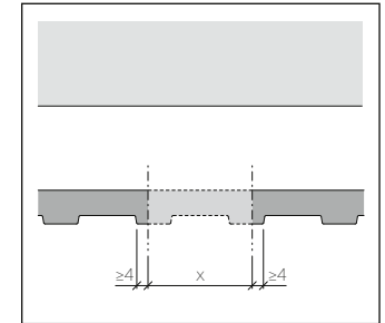
Onsite Gravial fabrication
