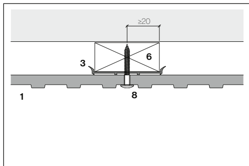
Timber Battens 60 mm Continuous Graviol grid
