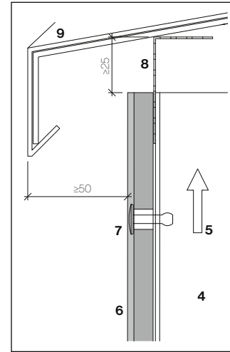
Sill detail
