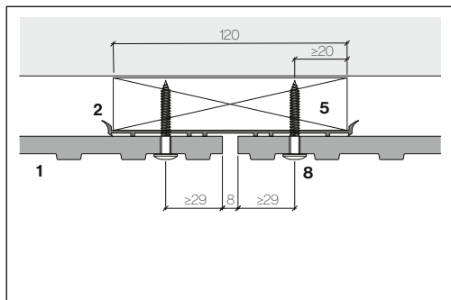
Timber Battens 120 mm Continuous Graviol grid
