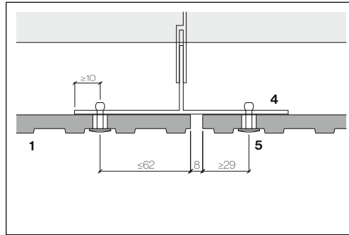
T-Profile 140 mm Individual Graviat grid
