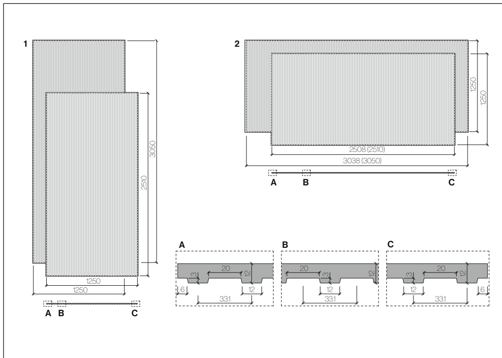
Graviol 9/12 mm thick panels - max. net panel sizes
